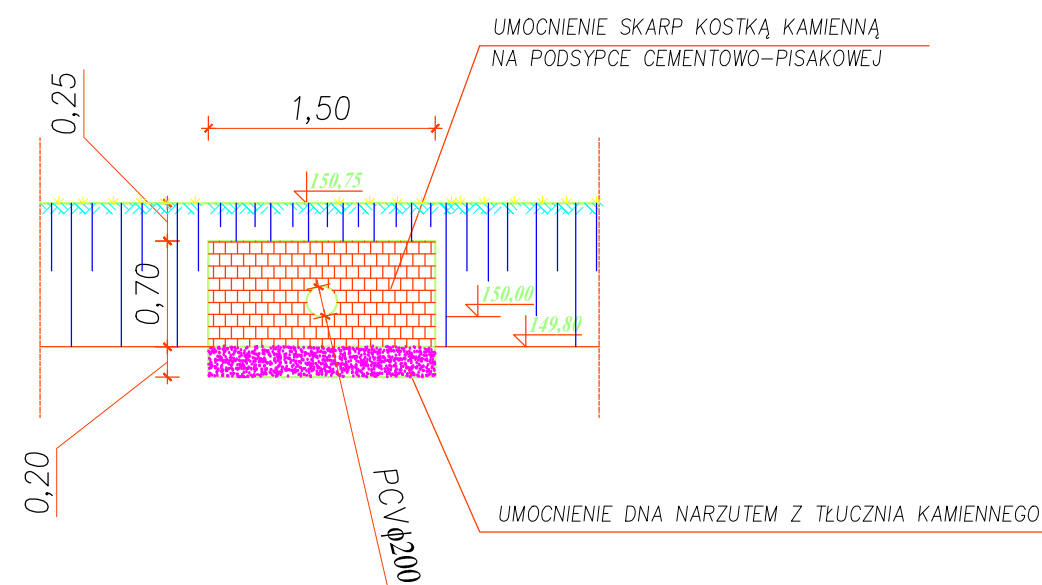
Wylot W3 km 1+255
